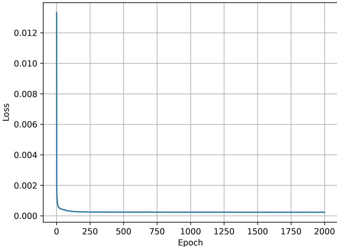
Training Loss - Fixed ENNC Architecture
